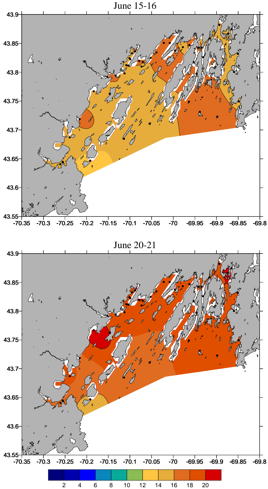
Figure 4. Surface water temperature ( ^{\circ}\text{C} ) on the June 15-16 and June 20-21, 2006 surveys. Station locations sampled denoted by black dots.
