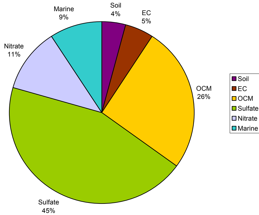
Figure 3-16. Mean composition of PM 2.5 aerosol by RCFM with marine (3.91 \mu\text{g}/\text{m}^3 ) at Acadia, March-May 1999-2001.
