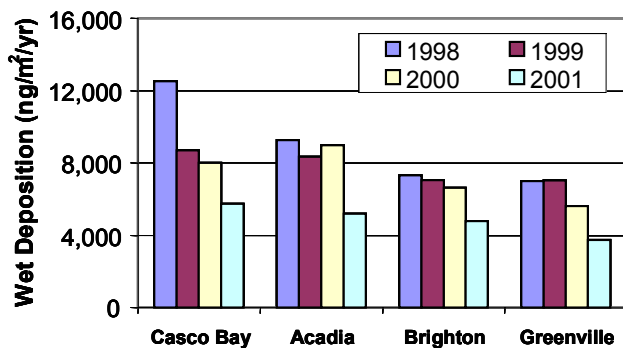
Figure 4-2. Annual 1998-2001 mercury wet deposition amounts ( \text{ng}/\text{m}^2 \text{ yr}^{-1} ) for sites in Maine.
