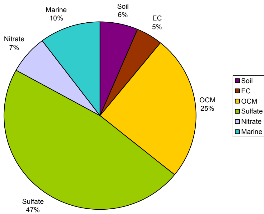
Figure 3-17. Mean composition of PM 2.5 aerosol by RCFM with marine (8.36 \mu\text{g}/\text{m}^3 ) at Acadia, June-August 1999-2001.
