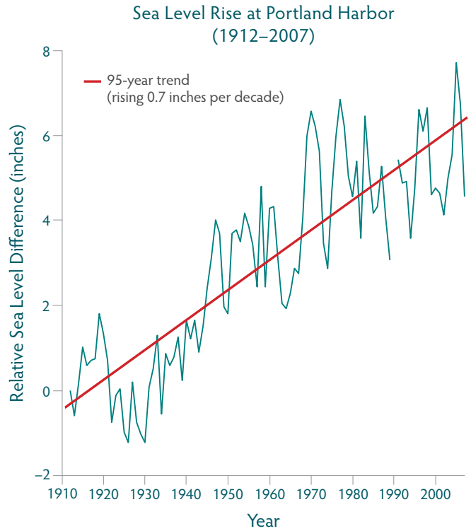
Relative sea level (inches) measured at the Portland Harbor tidal gauge, 1912 to 2007. The 1912 value has been subtracted from annual values to illustrate the change in sea level relative to the start of the record. The red line is the linear regression applied to the time series, and is used to calculate the rate of change: about 0.7 inches/decade (Wake et al. 2009).
